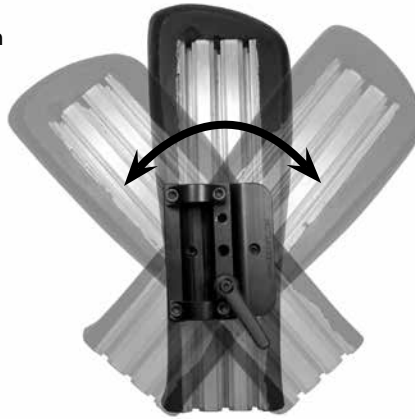
bottom view of armpad with swivel mount
